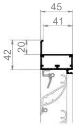
G 35Z Recessed wall louvre with flange
