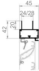
F 35Z Window louvre
