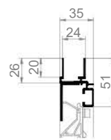
F 20Z Window louvre
