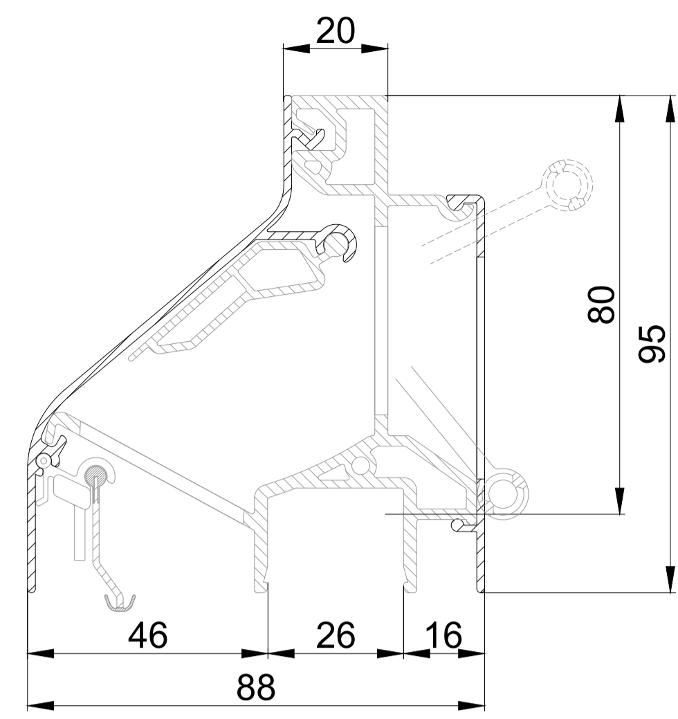
DucoLine 80 ZR / GG26
